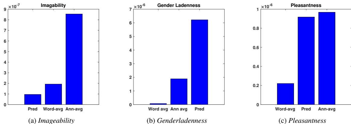
Fig. 4. MSE of predicted and baseline models in predicting Imageability, Genderladeness and Pleasantness
